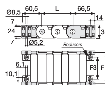
Fig. A Chain fixed inside/outside the radius. (Fig A)
