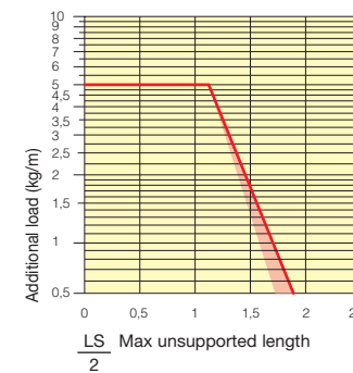
Fig. A Chain fixed inside/outside the radius. (Fig A)
