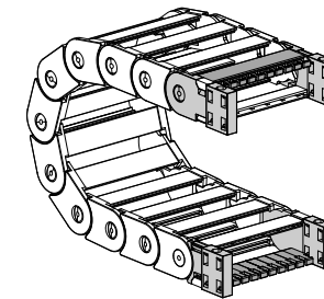
Fig. A Chain fixed inside/outside the radius. (Fig A)
